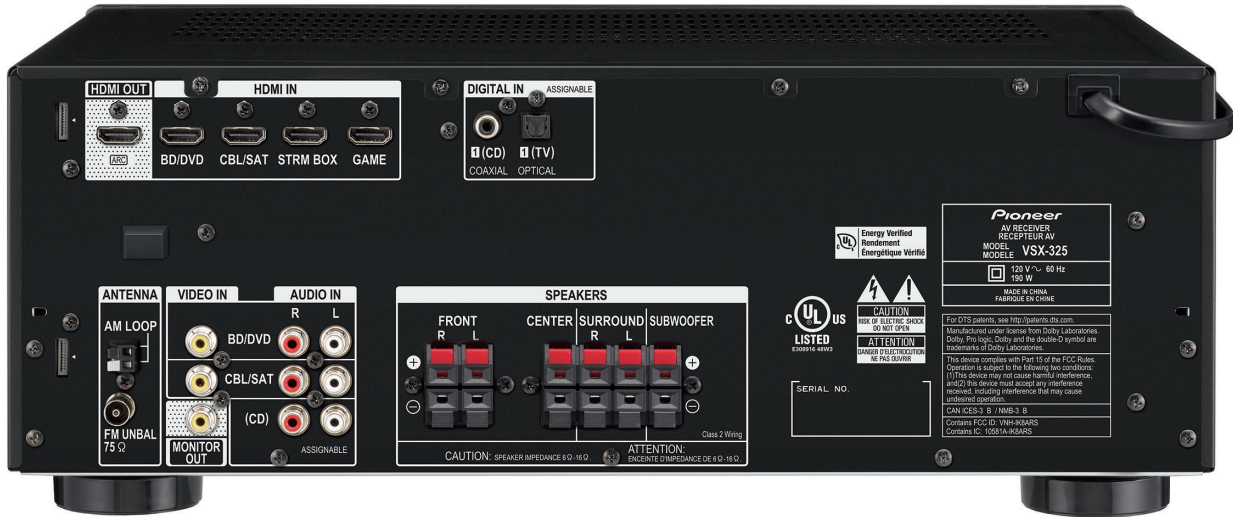
VSX-325 Rear Panel
